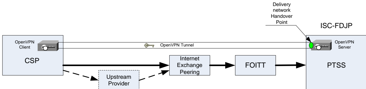
Figure 16-1: Schematic view of the OpenVPN delivery network
