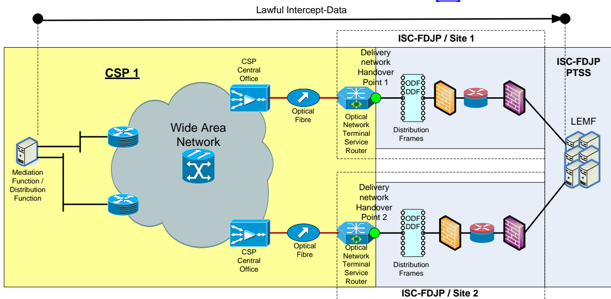
Figure 16-2: Schematic view of the direct connection to ISC-FDJP
