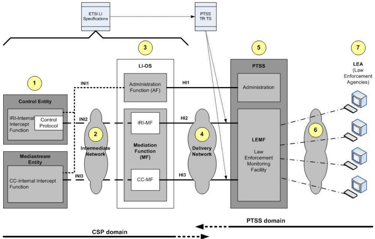
Figure 6-1: Lawful interception model for real-time interception
