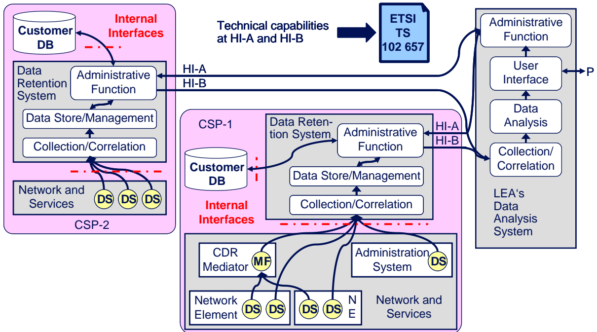
Figure 10-2: Retained Data functional architecture
