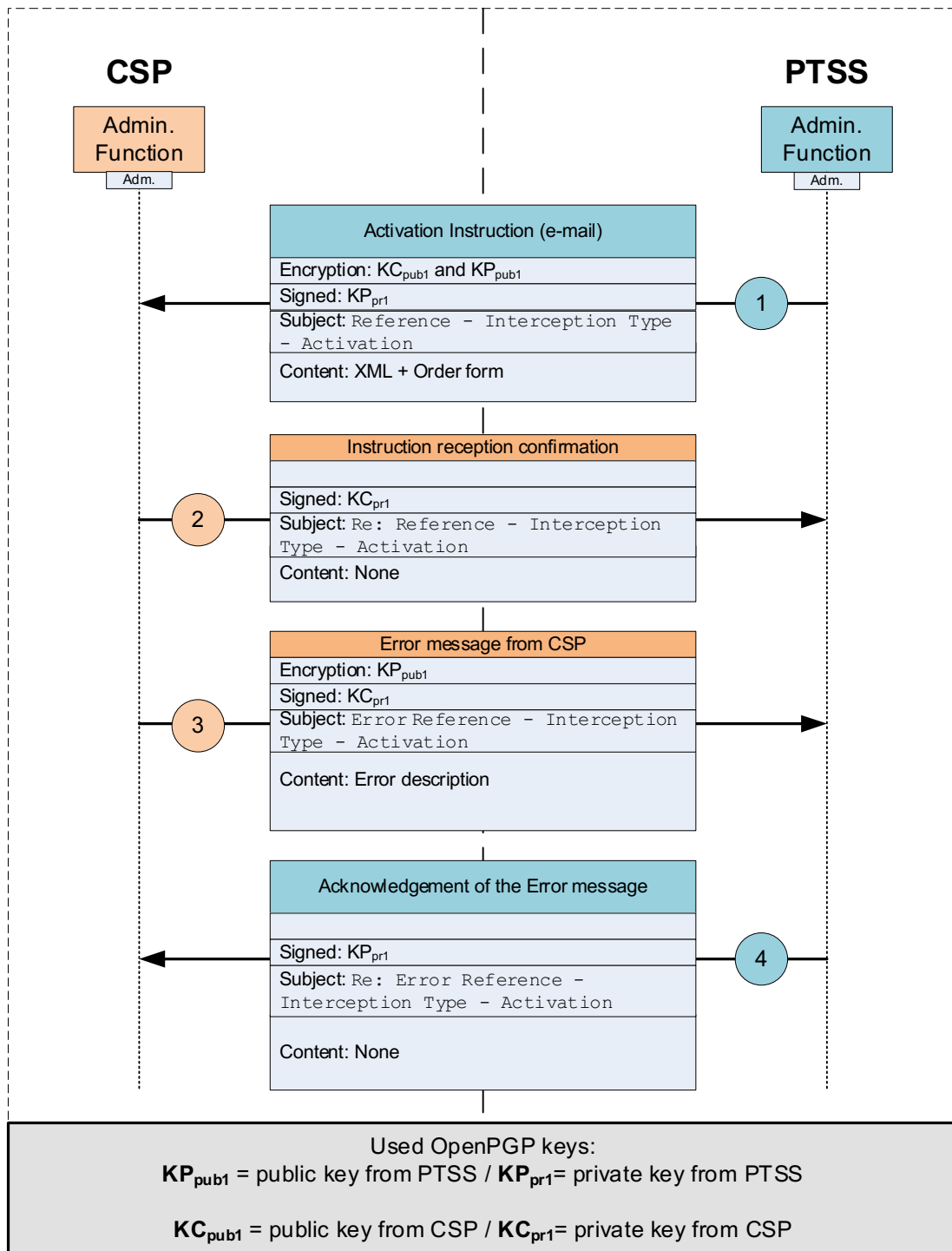
Figure 4-15: Message flow for error of email instruction activation processing for real-time interceptions
