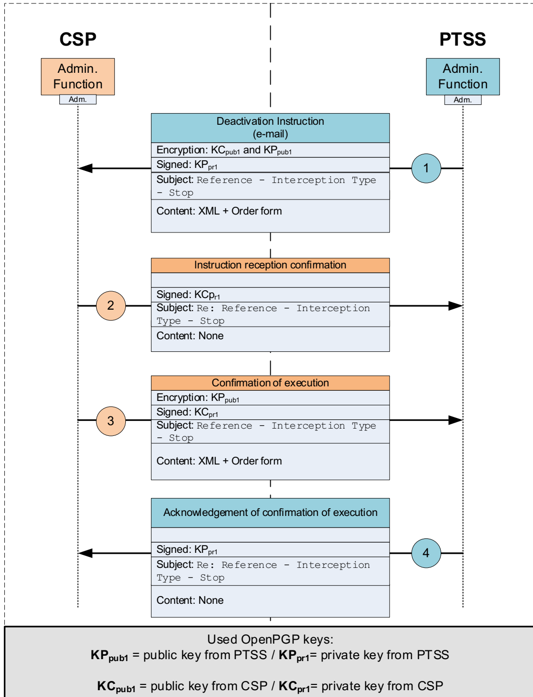
Figure 4-13: Message flow for email deactivation instruction processing for real-time interceptions
