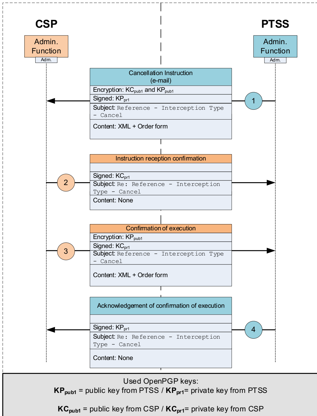
Figure 4-14: Message flow for email cancellation instruction processing for real-time interceptions
