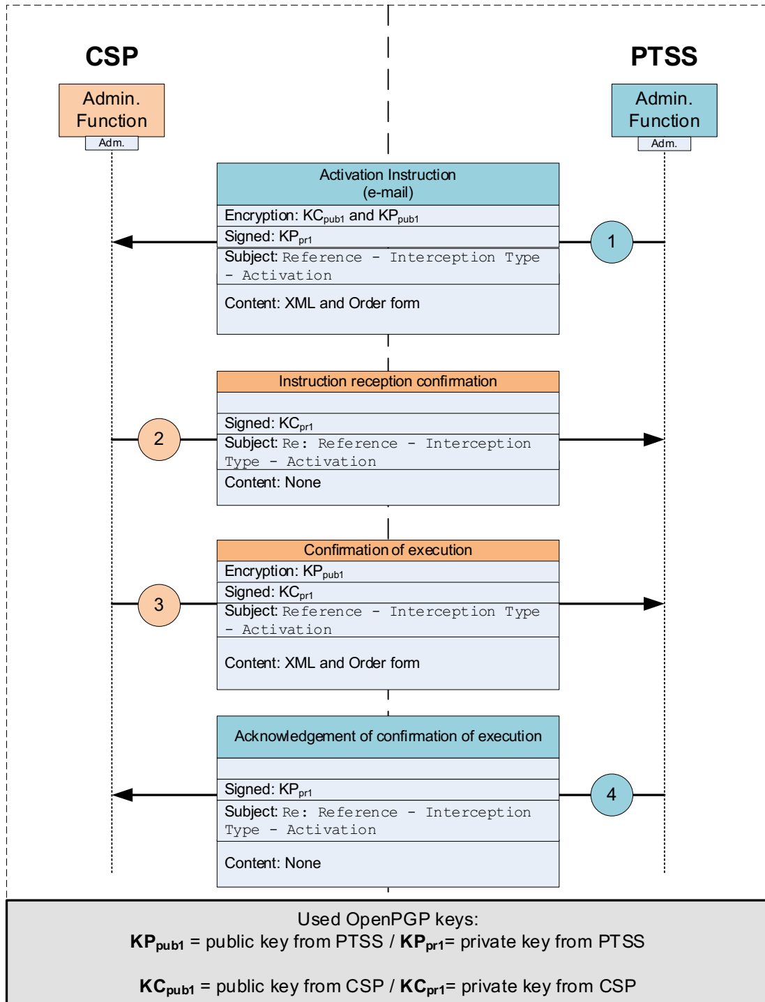
Figure 4-12: Message flow for email activation instruction processing for real-time interceptions
