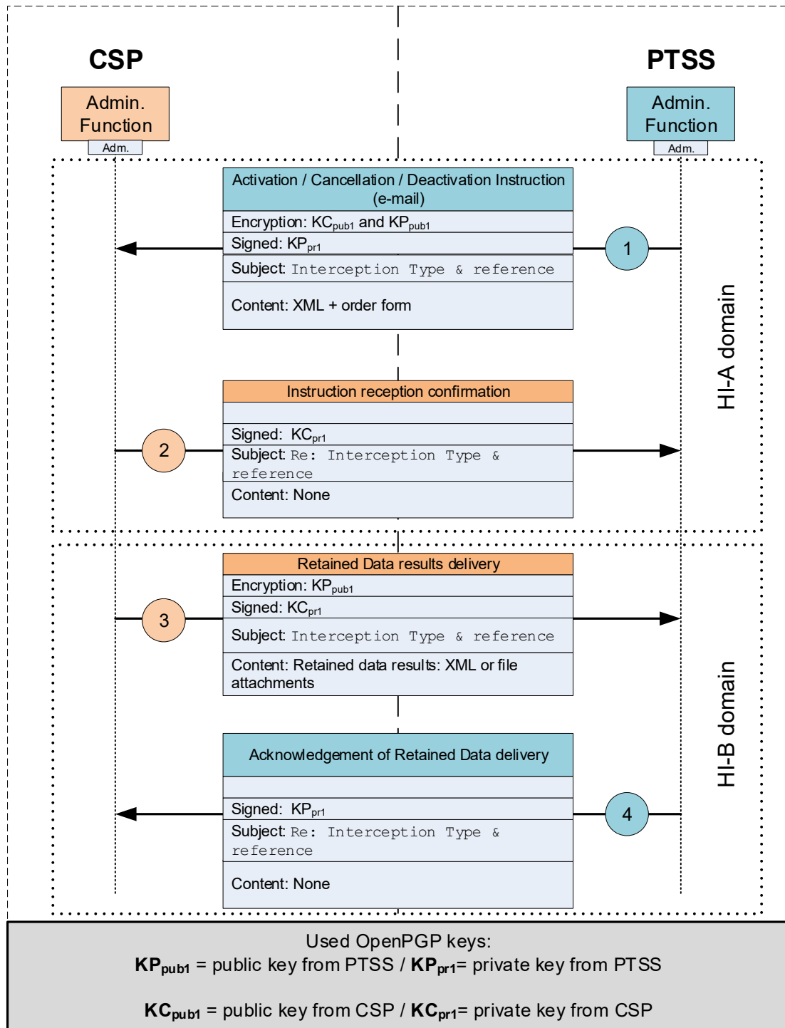
Figure 4-17: Message flow for secure email instruction processing for retained data
