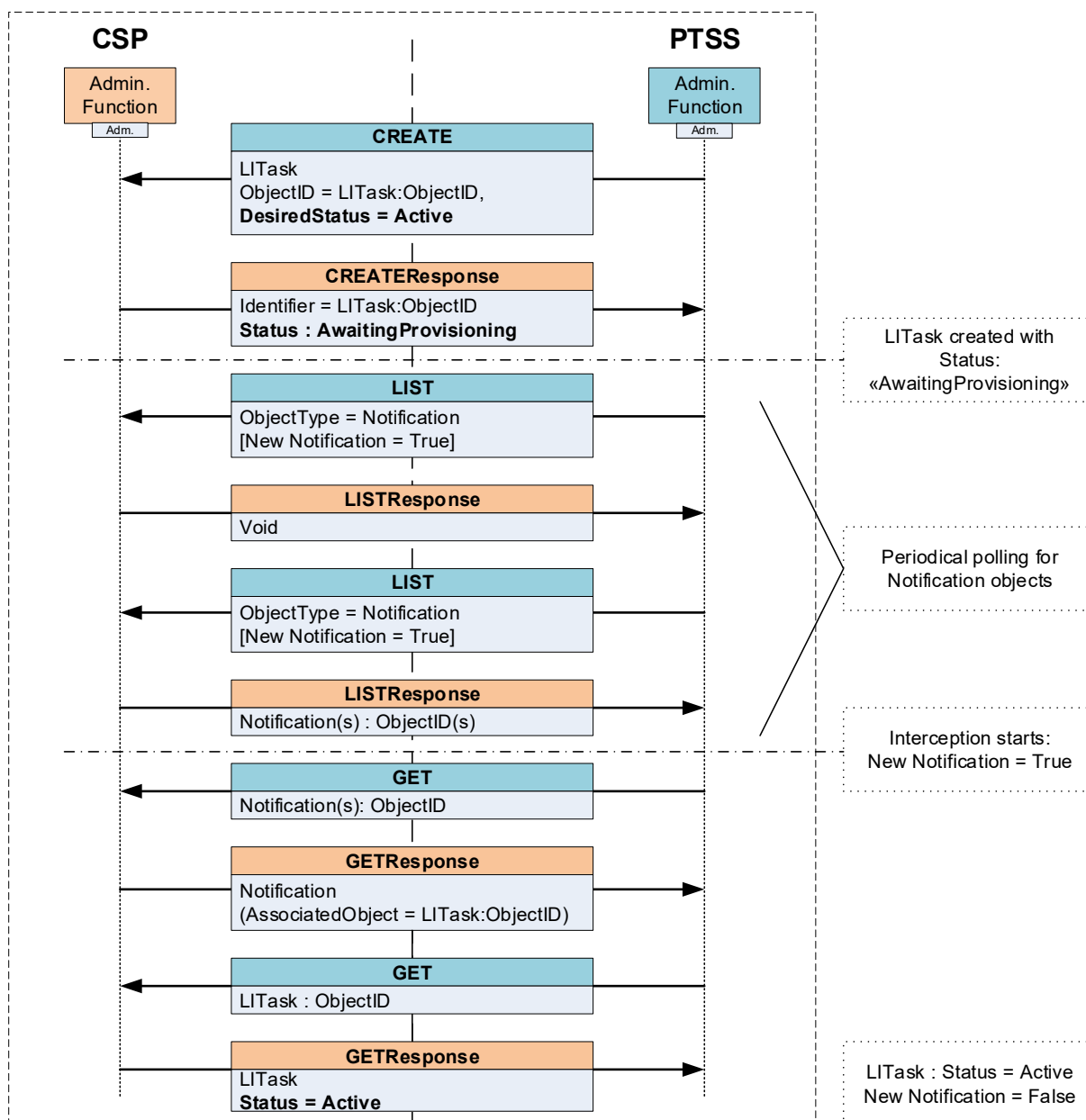
Figure 4-2: Message flow for a real-time interception activation instruction based on HTTP
