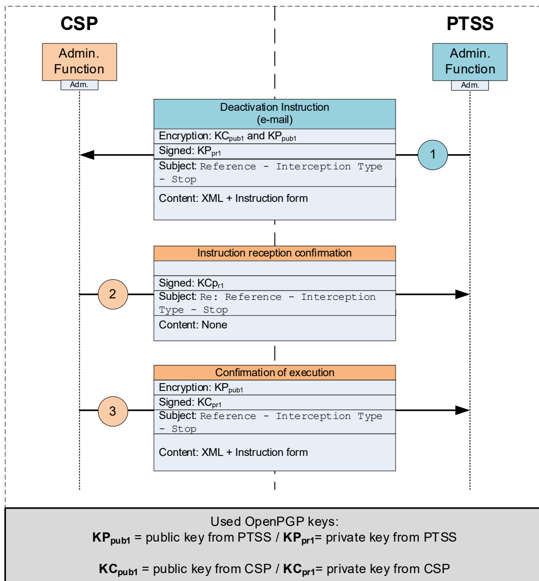
Figure 4-13: Message flow for email deactivation instruction processing for real-time interceptions
